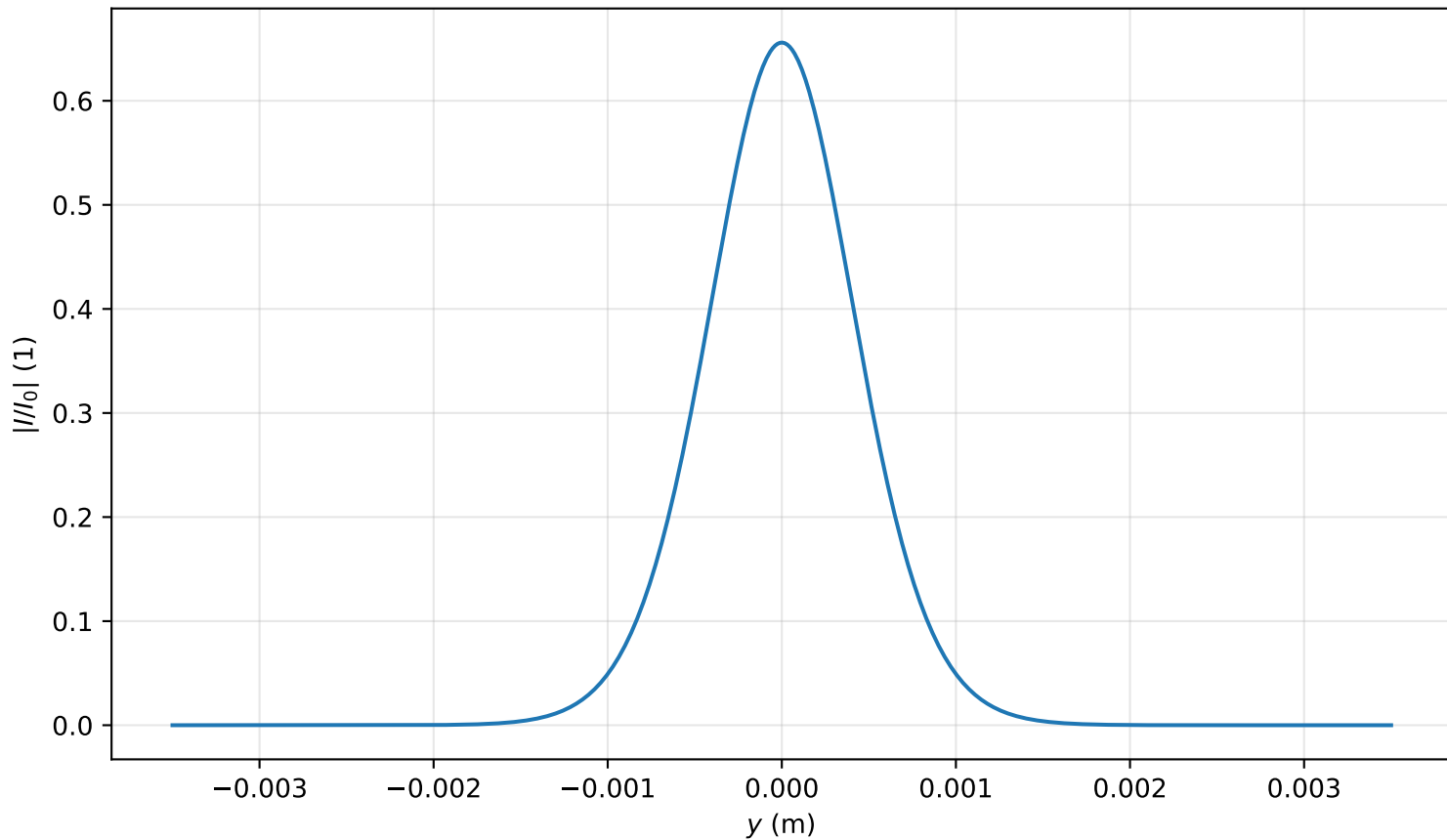
Intensity profile I(x=0, y, z=1.990)/I_0 , \text{Pin}=0.3\text{Pcr} , artificial time
